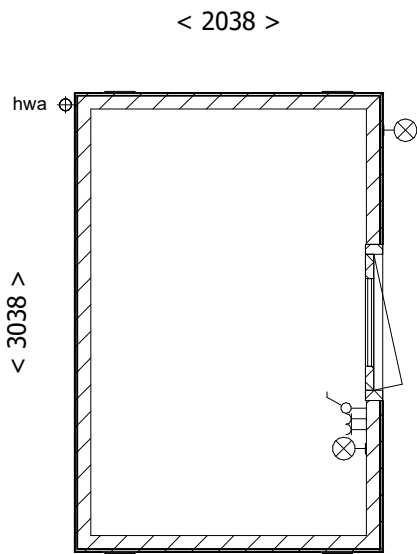
V0 = begane grond (Peil) 1 : 50
